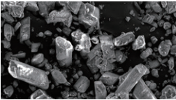
Conventional Sodium Bicarbonate Powder Average particle diameter: 73 µm Scanning electron microscope image magnification of 150 X
